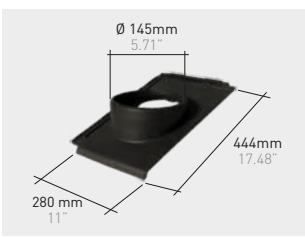
Q87*K | Planum chimney roof tile klinker
