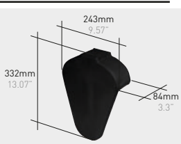
Q05*K | End cap / Straight gable end klinker
