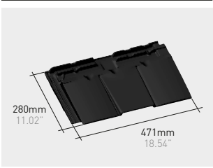
Q96*K | Visum3 ventilation roof tile klinker
